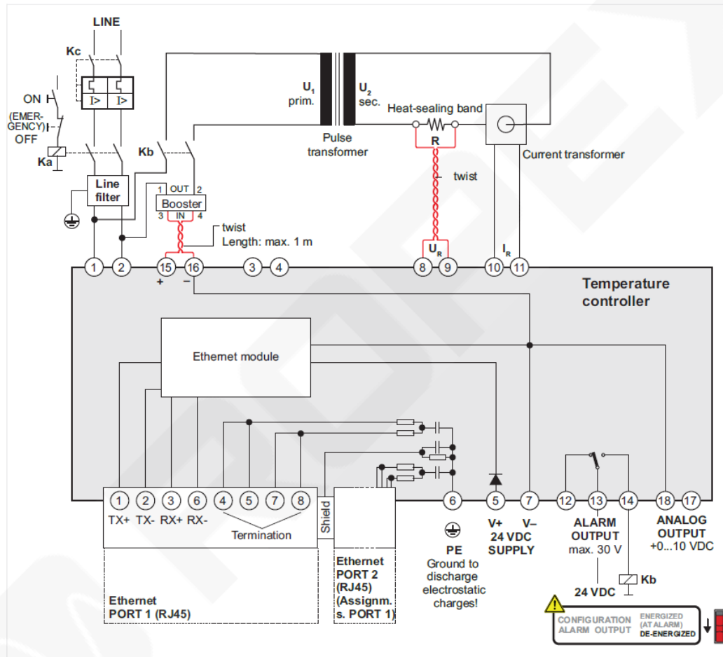
Illustration 6: Connection diagram, example of system with booster
