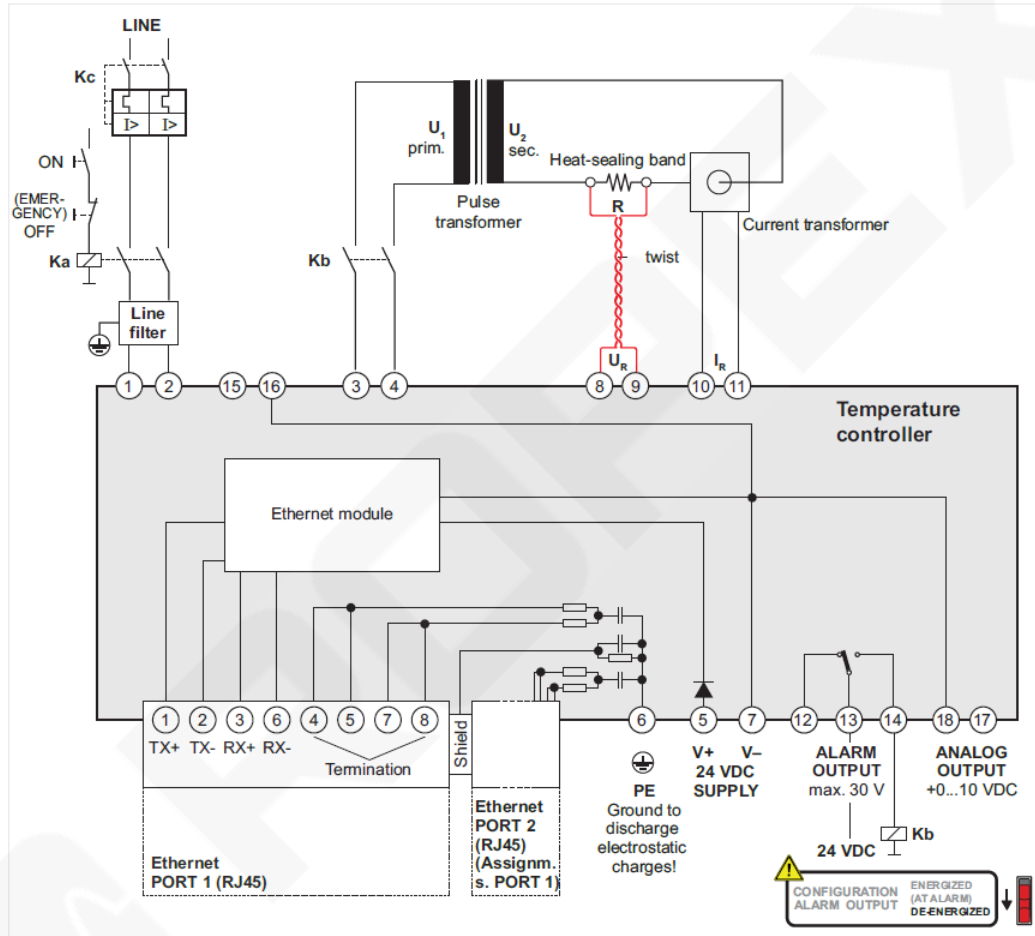
Illustration 5: Connection diagram, example of system without booster
